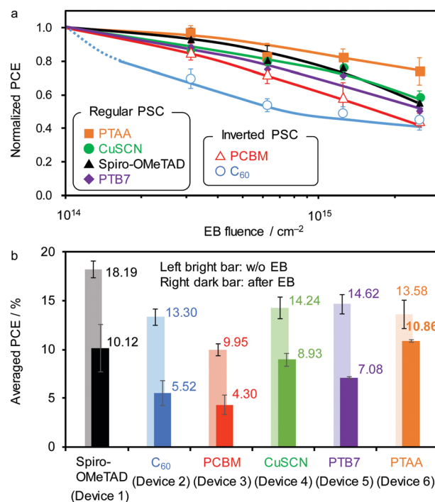
Fig. 5 (a) Normalized PCE of various PSCs upon EB exposure. (b) Average PCE values with error bars (standard deviation) before (left bar) and after EB exposure (right bar, F_{\text{EB}} = 2.5 \times 10^{15} \text{ cm}^{-2} exposure).
