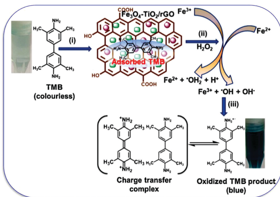
Fig. 12 The peroxidase-like activity of the FTG nanocomposite showing the (i) adsorption of TMB onto the FTG nanocomposite surface, (ii) formation of \text{OH}^\bullet by the Fenton reaction, and (iii) TMB oxidation by \text{OH}^\bullet radicals. 176 Copyright Elsevier B.V. 2019.
