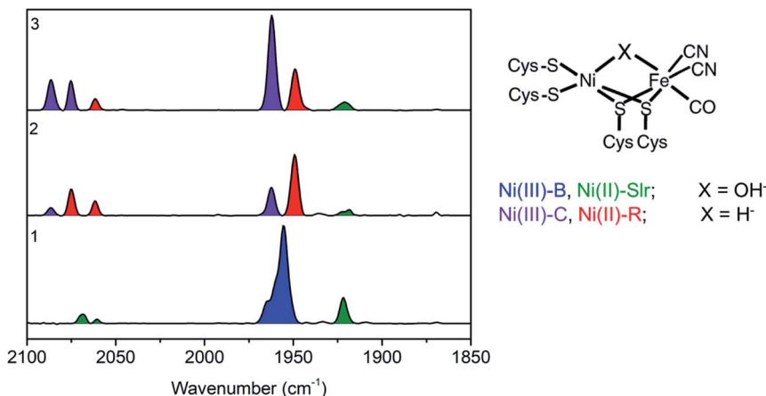
Fig. 2 (Left) Baseline corrected FTIR spectra of a Dv MF [NiFe] hydrogenase as isolated 1 , incubated 4 hours in \text{H}_2 atmosphere 2 , and in 15 \mu\text{l} of viologen and 40 \mu\text{l} NaDT 3 . Band positions for the different state are as follows: Ni(III)-B (1955, 2081, and 2090 \text{cm}^{-1} ), Ni(II)-Slr (1922, 2061, 2070 \text{cm}^{-1} ), Ni(III)-C (1961, 2074, 2085 \text{cm}^{-1} ), Ni(II)-R (1948, 2061, 2074 \text{cm}^{-1} ). (Right) Schematic representation of Dv MF [NiFe] hydrogenase active site, where X is identified for each redox state.
