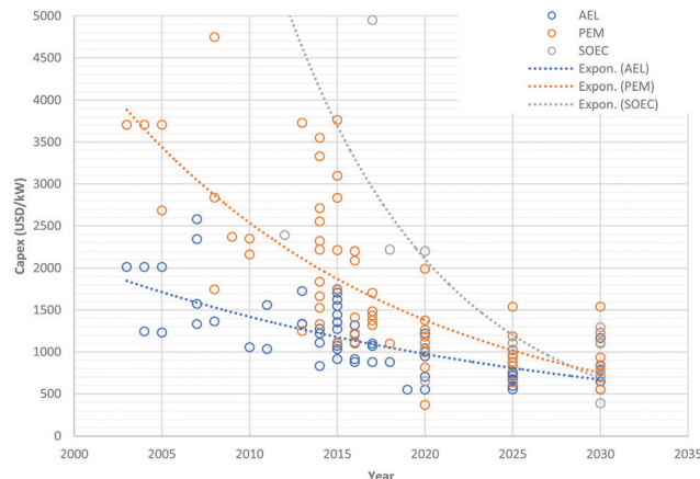
Fig. 6 Examples of CAPEX estimates for different electrolyser types for the year of development. Source: Glenk & Reichelstein. 155
