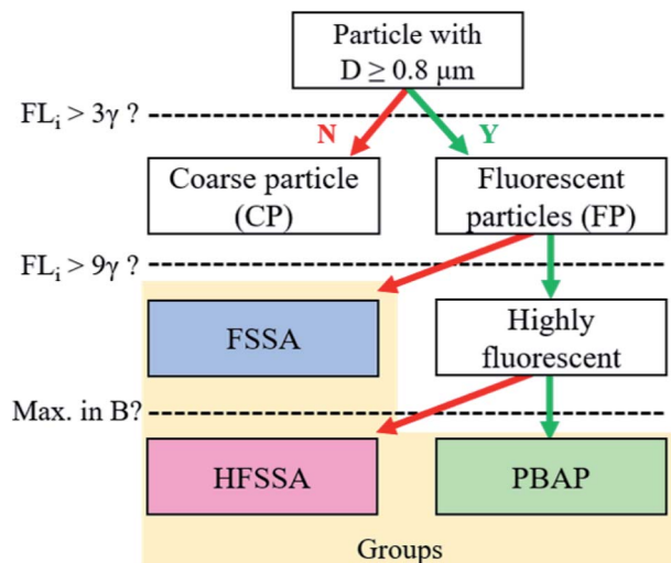
Fig. 2 Decision tree for classification of fluorescent particles. Particles with diameters larger than 0.8\ \mu\text{m} and with a fluorescent signal exceeding the 3\gamma -threshold at any detector channel are labelled as fluorescent particles (FP). FP whose fluorescent signal exceeds 3\gamma but not the 9\gamma -threshold are grouped as fluorescent sea spray aerosol (FSSA). Those that exceed the 9\gamma threshold are grouped as highly fluorescent sea spray aerosol (HFSSA) or as primary biological aerosol particles (PBAP) if their maximum fluorescent signal is observed in the B channel.
