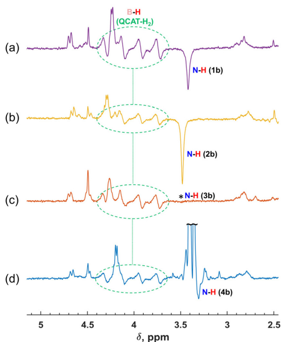
Fig. 2 (a)–(d) ^1\text{H} NMR spectra showing enhanced resonances observed in the hydrogenations of imines 1a – 4a with \text{para-H}_2 over the QCAT catalyst at 340 K in \text{toluene-d}_8 , respectively. The spectra were measured at the first moments after introducing \text{para-H}_2 into the corresponding imine–QCAT solutions. Spectral regions with the B–H group signals of the QCAT- \text{H}_2 intermediate and the N–H signals of the amine products 1b – 4b are displayed. Dotted ovals highlight the B–H group signals of QCAT- \text{H}_2 . The positions of the amine products are shown with text labels. The position of the signal of the N–H group hydrogen of 3b disappeared after introducing \text{para-H}_2 , which is marked with an asterisk in (c).
