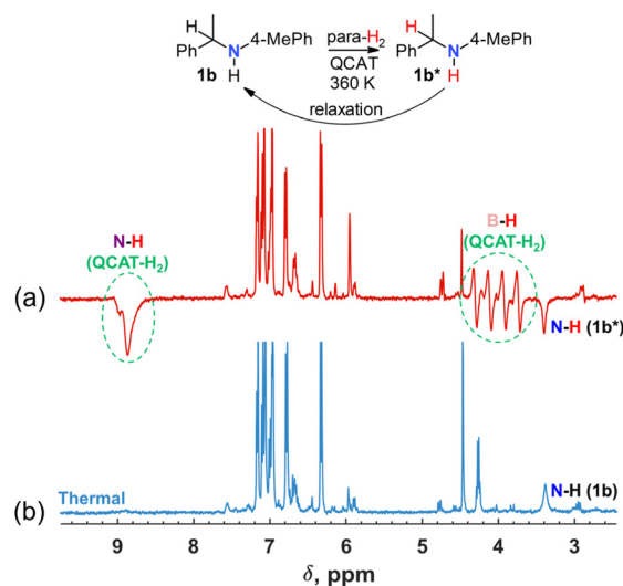
Fig. 3 ^1\text{H} NMR spectra acquired during the reaction of \text{para-H}_2 , QCAT and 1b . The red spectrum (a) was acquired using a \pi/4 pulse just after introducing \text{para-H}_2 into a solution containing 0.04 M QCAT and 0.04 M of 1b in \text{toluene-d}_8 at 360 K. The negative signal of the N–H proton of amine 1b is clearly visible. The signal of the \alpha -C–H hydrogen of 1b completely vanished, indicating a weak hyperpolarization of this group. The blue spectrum (b) was recorded after relaxation to the thermal equilibrium.
