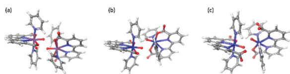
Fig. 7 Transition state structures of [Ru^V(bda)(py)_2-O]^+ dimer (a, O–O distance 1.9 Å), [Fe^V(bda)(py)_2-O]^+ dimer (b, O–O distance 2.1 Å) and 6-coordinate [Fe^V(bda)(py)_2-O]^+ dimer (c, O–O distance 2.0 Å).
