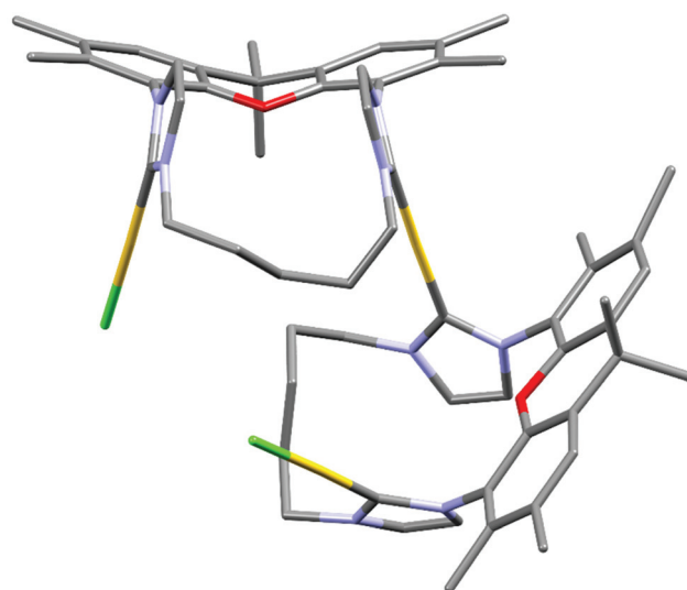
Fig. 4 X-ray crystal structure (sticks representation for improved clarity) of [\text{Au}(\text{AuCl})_2(\text{Cl})](\mathbf{16}) (colour code: Au yellow, Cl green, O red, N blue, H not displayed). Important bond lengths (pm) and angles (°): Au...Au 586.2(1), 572.8(1), 660.6(1), Au–C(NHC) 197(2), 198(2), 199(2), Au–Cl 28.4(4), 226.1(5); Cl–Au–C(NHC) 177.2(6), 178.2(6), C(NHC)–Au–C(NHC) 177.3(7).
