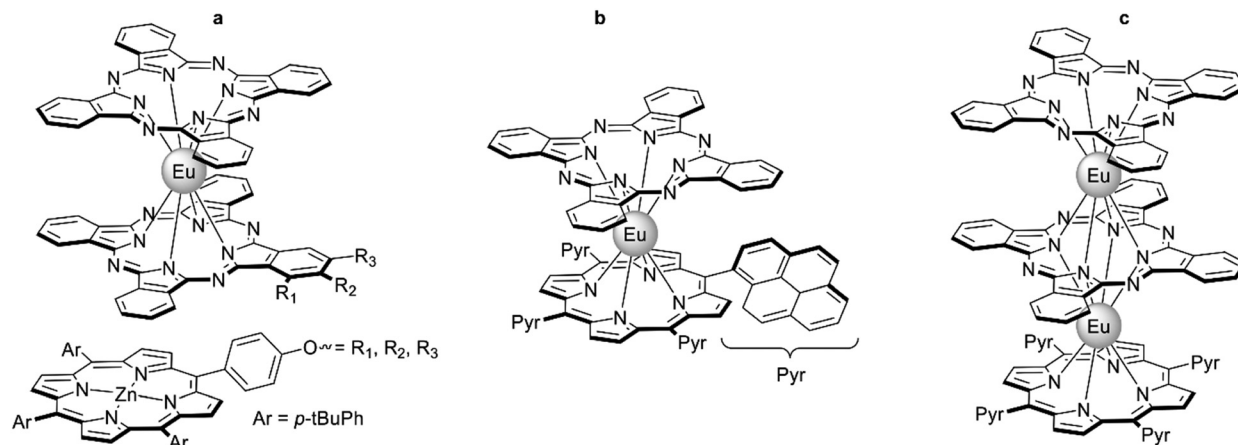
Fig. 42 Examples of \pi -extended sandwich complexes used for NLO studies: (a) Eu(III) bisphthalocyaninates with appended porphyrin units; 469 (b and c) double- and triple-decker complexes with meso -pyrenyl-substituted porphyrin ligands. 31
