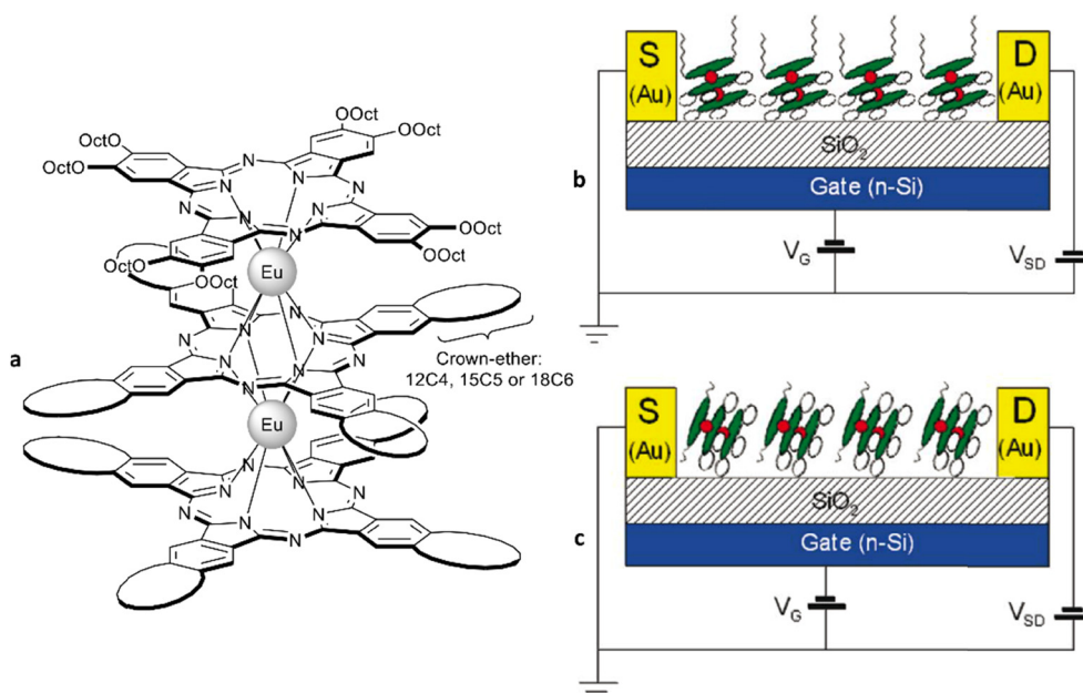
Fig. 36 (a) Amphiphilic Eu(III) crown-phthalocyaninates [(OctO)_8Pc]_3Eu[(crown)_4Pc]_3Eu[(crown)_4Pc] and schematic arrangement of complexes [(OctO)_8Pc]_3Eu[(12C4)_4Pc]_3Eu[(12C4)_4Pc] – (b) and [(OC_8H_{17})_8Pc]_3Eu[(18C6)_4Pc]_3Eu[(18C6)_4Pc] – (c) in the LB film-based OFET devices. Adapted with permission from ref. 439. Copyright 2009, American Chemical Society.
