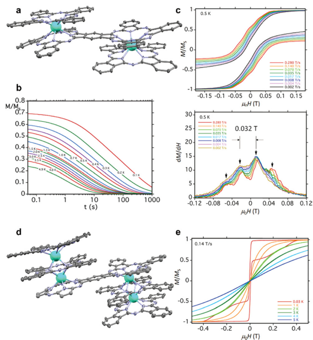
Fig. 23 Crystal structure of (a) (\text{Pc})\text{Ln}(\text{f-Pc})\text{Ln}(\text{Pc})^{\text{OBU}} (Ln 3+ = Dy and Tb) and (d) (\text{Pc})_2\text{Ln}_2(\text{f-Pc})\text{Ln}_2(\text{Pc})_2^{\text{OBU}} (Ln 3+ = Tb and Dy) and the micro-SQUID-measurement magnetization decay curves (b) and hysteresis loops for oriented crystalline samples of (c) (\text{Pc})\text{Tb}(\text{f-Pc})\text{Tb}(\text{Pc})^{\text{OBU}} and (e) (\text{Pc})_2\text{Dy}_2(\text{f-Pc})\text{Dy}_2(\text{Pc})_2^{\text{OBU}} . Molecular structures of (a) and (d) based on the cif files from ref. 217 and 220. Protons and n -butoxy groups in (\text{Pc})\text{Ln}(\text{f-Pc})\text{Ln}(\text{Pc})^{\text{OBU}} and (\text{Pc})_2\text{Ln}_2(\text{f-Pc})\text{Ln}_2(\text{Pc})_2^{\text{OBU}} are omitted for clarity. Adapted with permission from (a and b) ref. 217. Copyright 2018, American Chemical Society. Adapted with permission from (d and e) ref. 220. Copyright 2018, Wiley-VCH.
