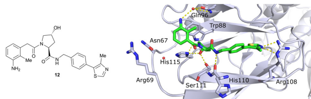
Fig. 6 Cocystal structure of inhibitor 12 bound to VCB (PDB 4B9K), derived from combinatorial optimisation of LHS and RHS. 13
