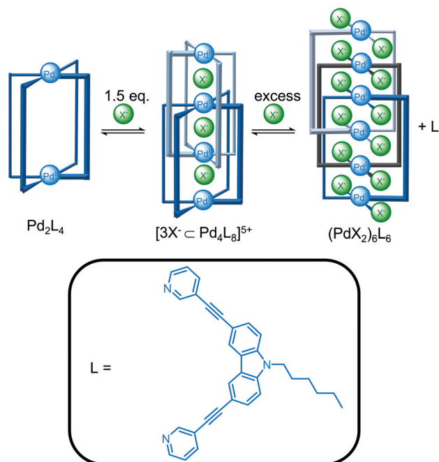
Fig. 3 Clever and co-workers' halide templated formation of a [\text{3X}^- \subset \text{Pd}_4\text{L}_8]^{5+} interpenetrated double cage from a [\text{Pd}_2\text{L}_4](\text{BF}_4)_4 cage and subsequent conversion to the triply catenated (\text{PdX}_2)_6\text{L}_6 upon addition of excess halide ions.
