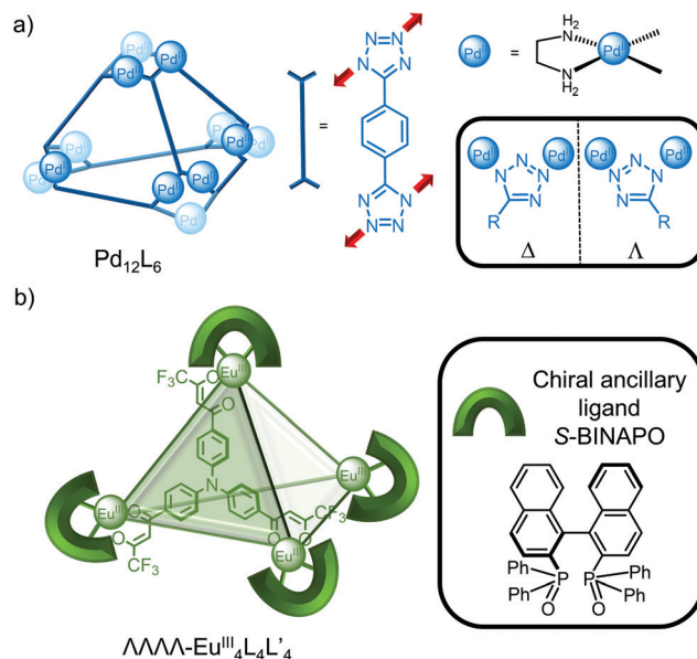
Fig. 4 Homochiral cages: (a) Mukherjee and co-workers' \text{Pd}_{12}\text{L}_6 tetrahedral cage with unusual homochirality due to symmetry breaking of the ligand upon metal coordination in the 1,3-binding mode. Inset: \Delta and \Lambda configurations; (b) Li and Yan's enantiopure \text{Eu}^{\text{III}}_4\text{L}_4\text{L}'_4 cage where the chiral ancillary ligand ( \text{L}' = \text{S-BINAPO} ) induces the chirality.
