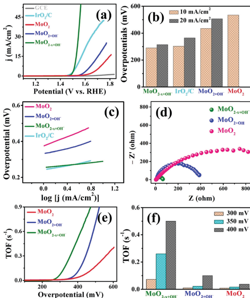
Fig. 27 Polarisation curves toward the OER for as-grown \text{MoO}_{2+\text{OH}^-} (7 h case), \text{MoO}_{2-x+\text{OH}^-} (9 h case), commercially available \text{MoO}_2 , and \text{IrO}_2/\text{C} electrocatalysts on GCE in 1 M KOH electrolyte. Reproduced with permission from ref. 531. Copyright American Chemical Society 2020.
