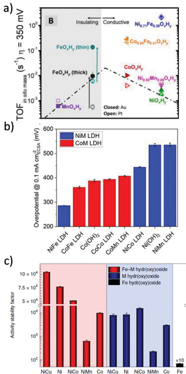
Fig. 51 Transition metal (oxy)hydroxides and LDHs OER performance trends. (a) Activity trend as effective turnover frequencies (TOF) at overpotential \eta = 350 \text{ mV} and based on the total mass of the electrodeposited catalyst films calculated from quartz crystal microbalance measurements and ordered based on the atomic number of the host/primary metal cation. Electrolyte: 1 \text{ M KOH} . Reproduced from ref. 826. Copyright American Chemical Society 2015. (b) Intrinsic activity trend as OER overpotentials at ECSA-normalised current densities of 0.1 \text{ mA cm}^{-2} ECSA for crystalline transition metal LDHs. Electrolyte: 0.1 \text{ M KOH} . Reproduced from ref. 831. Copyright Wiley 2021. (c) Activity stability factor (ASF) trend for Fe containing (red bars) and Fe-free (blue bars) transition metal hydroxy oxide clusters. The Fe containing catalysts were obtained by adding Fe nitrate to the 0.1 \text{ M KOH} electrolyte. Reproduced with permission from ref. 827. Nature Publishing 2020.
