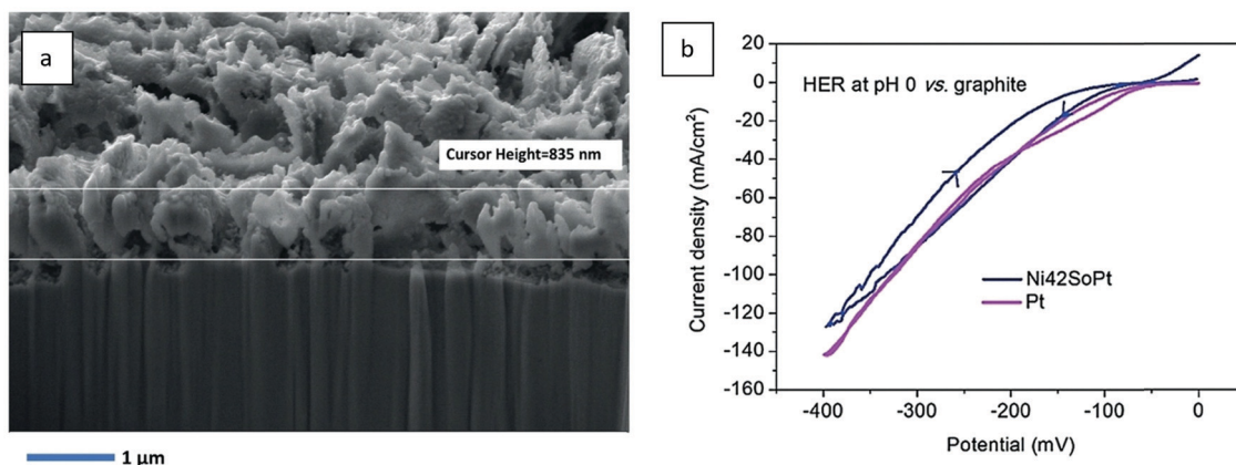
Fig. 106 (a) SEM photograph showing the cross-section of the Ni 42 /Pt interface (Pt thickness ~800–900 nm); the Pt loading is 1.8 mg cm -2 . (b) comparison of the HER performances of Pt and Ni 42 SoPt at pH = 0. Reproduced with permission from ref. 1269. Copyright Wiley 2019.
