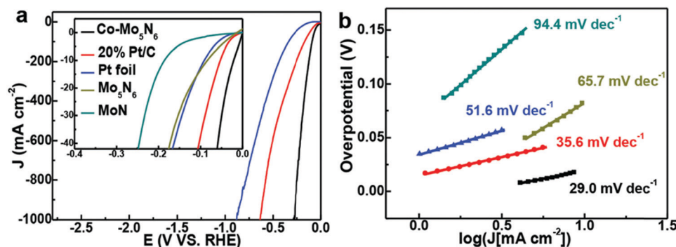
Fig. 68 Electrochemical measurements. (a) HER polarisation curves of the samples in 1.0 M KOH. (b) Corresponding Tafel plots. Reproduced with permission from ref. 1031. Copyright Wiley 2020.
