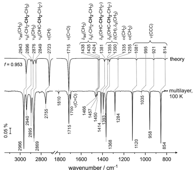
Fig. 1 Calculated gas-phase spectrum of butanal at the DFT-B3LYP level of theory (upper spectrum) compared to the IR spectrum of butanal adsorbed on pristine Pd(111) at 100 K at multilayer coverage (bottom spectrum). The multilayer spectrum was obtained in a flux of 5.1 \times 10^{13} \text{ mol cm}^{-2} \text{ s}^{-1} and a resulting exposure of 1.7 \times 10^{16} \text{ mol cm}^{-2} .
