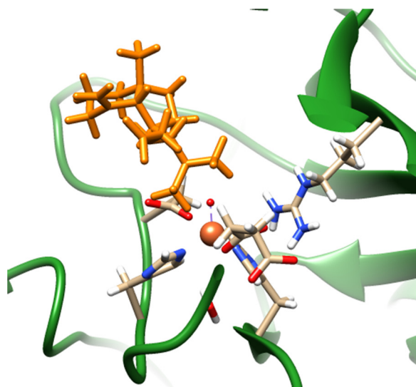
Sn 91.86 from MD with substrate \gamma -Gly-A
