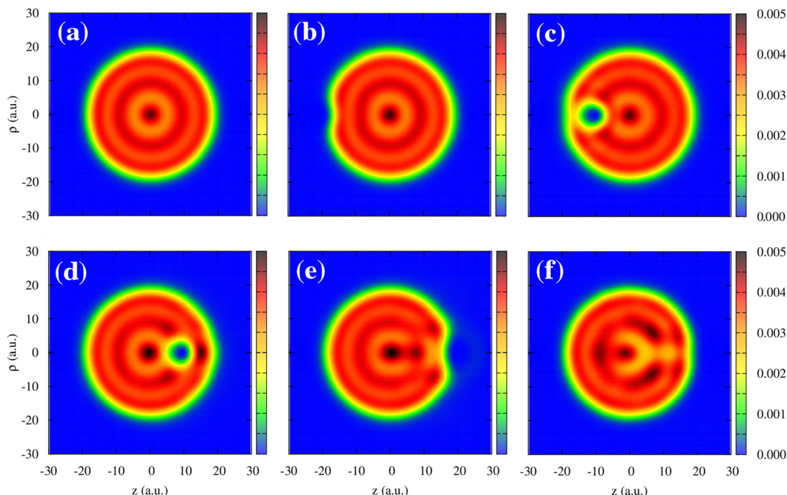
Fig. 6 Electron density of the \text{Na}_{106} cluster (radius R_{\text{cl}} = 18.93 a.u.) upon collision with antiproton. Results are shown as a function of the cylindrical ( z , \rho ) coordinates. The projectile moves with the constant velocity \nu = 0.3 a.u. along a straight-line trajectory following the symmetry z -axis of the system that passes through the center of the cluster. The snapshots correspond to six different antiproton positions: (a) z_p = -30 a.u., (b) z_p = -20 a.u., (c) z_p = -10 a.u., (d) z_p = 10 a.u., (e) z_p = 20 a.u., and (f) z_p = 30 a.u. The color code shows the electron density of the cluster in electrons per (a.u.). 3
