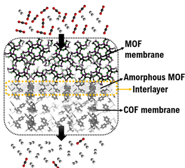
Fig. 3 Schematic representation of MOF/COF composite membrane. The amorphous MOF formed in the interlayer filled the free spaces between COF crystals and the interface between COF and MOF layers. The figure was adapted from the literature with permission from ref. 34. Copyright (2016) American Chemical Society.
