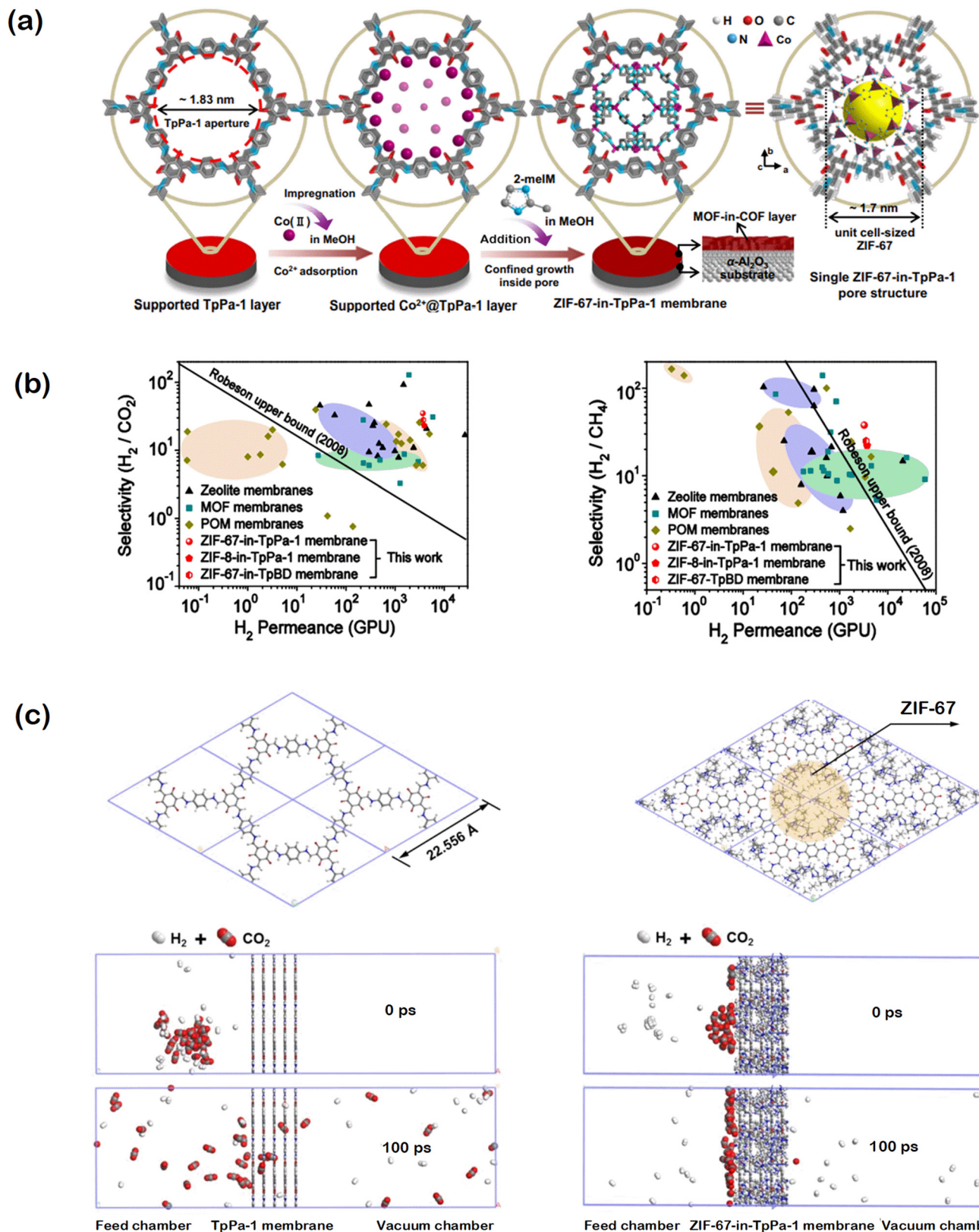
Fig. 5 (a) Representation of MOF-in-COF (ZIF-67-in-TpPa-1) structure. In the impregnation step, the supported TpPa-1 layer was immersed in cobalt nitrate hexahydrate solution and then 2-methylimidazole (2-melm) solution. Reprinted with permission from ref. 41. (b) Comparison of H_2 permeance, H_2/CO_2 and H_2/CH_4 selectivities of MOF-in-COF membranes with those of traditional membranes. Reprinted with permission from ref. 41. (c) Simulation system to depict H_2/CO_2 permeation through pure TpPa-1 membrane and ZIF-67 incorporated TpPa-1 membrane. Reprinted from ref. 41 under the terms of the CC BY licence https://creativecommons.org/licenses/by/4.0/ .
