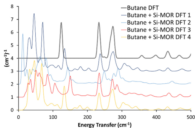
Fig. 2 Comparing the calculated INS spectra of n -butane in siliceous mordenite for a range of geometries. In all cases, the experimental shifts of the butane torsional modes to lower energy values, on encapsulation in the mordenite pore (Fig. 1) were not replicated. See text for further details. Data is artificially incremented by 1\text{ (cm}^{-1})^{-1} for ease of reading.
