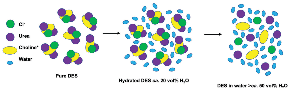
Fig. 16 Cartoon diagram showing structural changes in a DES starting with the pure choline \text{Cl}^- :urea DES (left). As the water content increases the hydrated DES regime is reached (middle, ca. 20 vol%), then the high concentration regime where everything is fully hydrated (ca. 50 vol%). Reprinted with permission from Elsevier. 207
