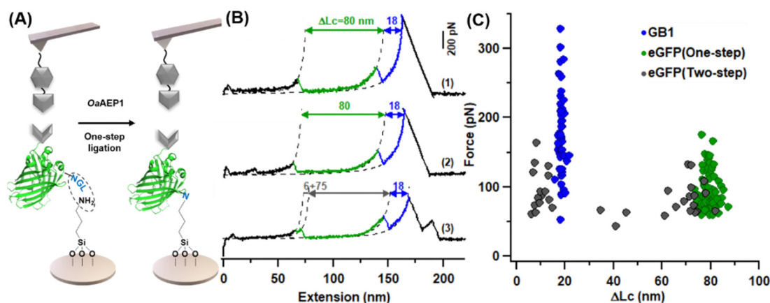
Fig. 4 One-step immobilization of eGFP for AFM-SMFS study. (A) Scheme of AEP-mediate eGFP immobilization on the amino-functionalized glass surface. (B) Representative force-extension curves showing different unfolding pathways of GFP: one-step (traces 1 and 2) and two-step (trace 3). (C) Scatter plots of F - \Delta L_c of fused protein showed expected unfolding results for eGFP.
