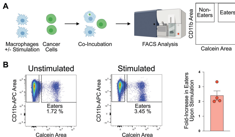
Fig. 1 Macrophage phagocytosis increases with interferon-gamma (IF- \gamma ) treatment. (A) Donor-derived macrophages are stimulated with IF- \gamma (72 h, R&D Systems) or PBS control prior to co-incubation with calcein stained SW620s (2 h). Cell populations are analyzed via flow cytometry for CD11b and calcein intensity. (B) Stimulated macrophages show a 2.41 \pm 0.62 -fold increase in Eaters upon IF- \gamma treatment across 4 replicates.
