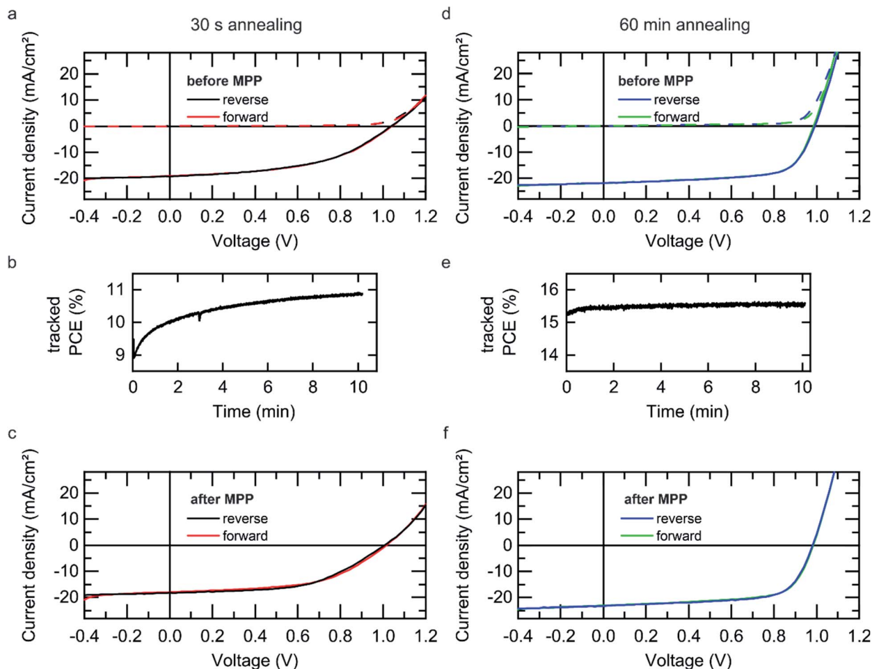
Fig. 8 MPP tracking under 1 sun illumination. (a) Initial J-V curves of a solar cell that was annealed for 30 s. (b) The PCE increases significantly during MPP measurement. (c) After MPP-tracking, the J-V curves of the solar cell revert back to their initial shape. (d–f) After 60 min of thermal annealing, the PCE of a solar cell remains constant during MPP-tracking and the J-V curves persisted.
