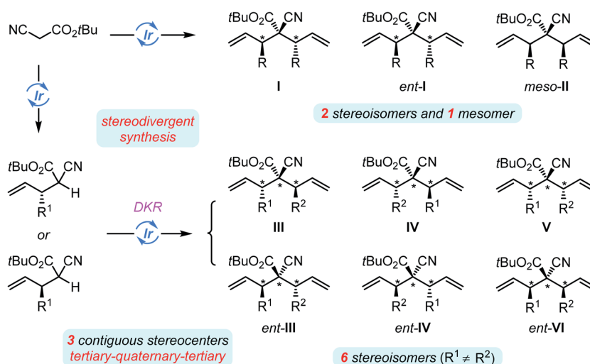
Scheme 2 Ir-catalyzed double-asymmetric allylic alkylation ((a) previous work) and stereodivergent double allylation ((b) this work).
