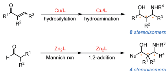
Scheme 1 Two conceptually distinct stereodivergent syntheses with dual catalysis (a) and single catalysis (b).
