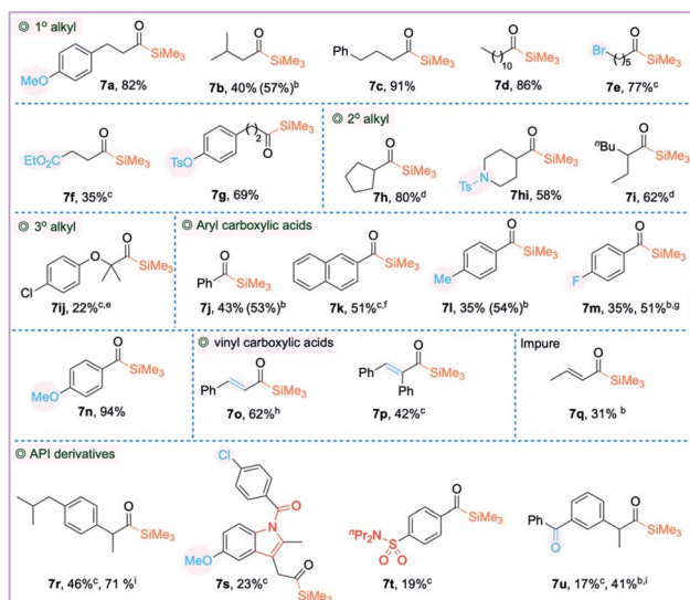
\begin{array}{ccc} \text{R}-\text{C}(=\text{O})\text{OH} & \xrightarrow[\text{DMF (20 mol\%), DCM}]{\text{i. (COCl)}_2 \text{ (3.0 eq.)}} & \text{R}-\text{C}(=\text{O})\text{SiMe}_3 \\ \text{3} & \xrightarrow[\text{DME, rt, 12 h}]{\text{ii. Ni(OAc)}_2 \cdot 4\text{H}_2\text{O (10 mol\%)}, \text{dtbpy (10 mol\%)}, \text{Me}_3\text{SiZnI (1.2 eq.)}} & \text{7} \end{array} R = alkyl/aryl/alkenyl
