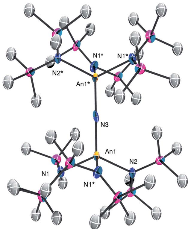
Fig. 1 Solid-state molecular structure of 2 shown with 50% probability ellipsoids. [\text{K}(\text{18-crown-6})(\text{THF})_2]^+ counterion and hydrogen atoms are removed for clarity.
