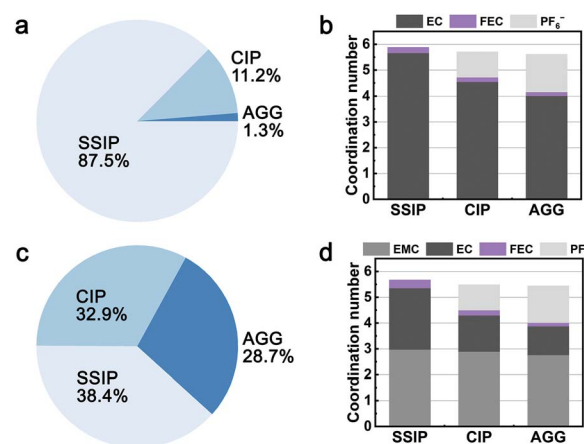
Fig. 4 The population and species-specific coordination number of SSIP, CIP, and AGG in (a and b) the ECF electrolyte and (c and d) the GenF electrolyte.
