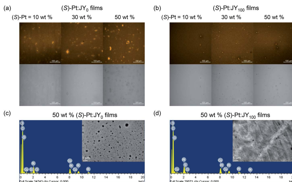
Fig. 7 (a and b) Confocal laser-scanning fluorescence micrographs ( \lambda_{\text{ex}} = 405 nm, \lambda_{\text{obs}} = 500\text{--}700 nm) for JY 0 (a) and JY 100 (b) films (quartz substrates) doped with various concentrations (10, 30 and 50 wt%) of (S)-Pt: top panels, fluorescence images; bottom panels, bright-field images. Scale bar = 100 \mu\text{m} . (c and d) Energy dispersive X-ray spectra and the average atomic percentage compositions of JY 0 (c) and JY 100 (d) films doped with 50 wt% (S)-Pt (200 mesh carbon films on copper). The atomic percentage compositions of Pt were quantified for Cliff Lorimer thin ratio sections: 1.4% Pt for (S)-Pt:JY 0 films; 1.5% Pt for (S)-Pt:JY 100 films. The insets show TEM images of the JY films doped with 50 wt% (S)-Pt. Scale bar = 1 \mu\text{m} .
