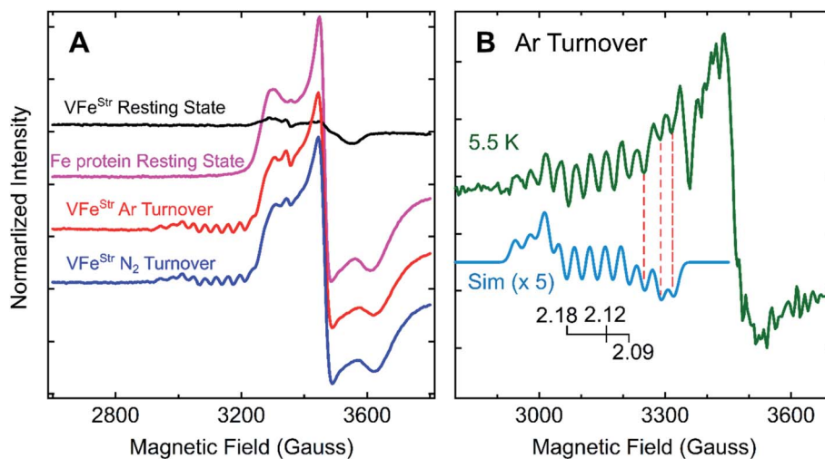
Fig. 5 g -2 region X-band EPR spectra of V-nitrogenase proteins. (A) 12 K spectra of resting states (black trace for VFe Str and magenta trace for Fe protein) and Fe protein-VFe Str freeze-trapped during turnover under Ar (red trace) and N 2 (blue trace) (B) 5.5 K (green trace) spectra of Ar-turnover Fe protein-VFe Str along with simulation of turnover intermediate (cyan trace) with 51 V hyperfine coupling, a_{\text{iso}} = 110 MHz, g = [2.18, 2.12, 2.09] , and isotropic EPR linewidth of 75 MHz. Samples: all samples contain 5 \mu\text{M} of VFe Str protein except the Fe protein resting state sample, and 40 \mu\text{M} of Fe protein except the VFe Str resting state sample. All samples made in buffer with 200 mM MOPS at pH 7.3 and an ATP-regeneration system (20 mM ATP, 20 mM MgCl 2 , 1 mg mL -1 BSA, and 0.4 mg mL -1 creatine phosphokinase) with a final dithionite concentration at \sim 20 mM. EPR conditions: as in Fig. 3 except each spectrum is the sum of 10 scans.
