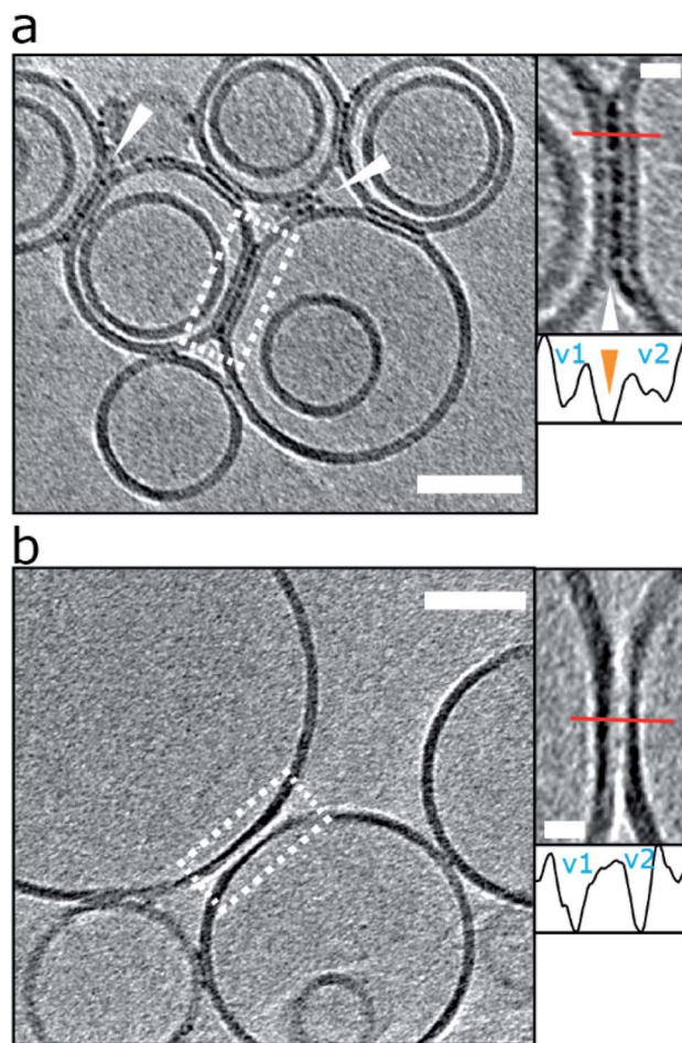
Fig. 6 Liposomes can be linked together by A \beta 42 protofibrils. (a) For preparation with reduced levels of A \beta 42 oligomer/protofibrils, A \beta 42 assemblies become localized to inter-vesicular space and connect the membranes of neighbouring vesicles (arrowheads). In preparations of reduced levels of oligomer/protofibrils, A \beta 42 decoration is not observed elsewhere on the vesicles. Area rimmed in white is shown with more detail in inset on the right. Profile plots along the red lines indicate the presence of additional density (orange arrowhead) between the two vesicles marked as v1 and v2. (b) Control experiment showing vesicles with no A \beta 42 added. Please note the absence of additional densities in areas where vesicles are in contact. The tomographic slices are 7.6 nm thick with scale bars: 50 nm, insets: 10 nm. Similar supporting data is shown in Fig. S9.†
