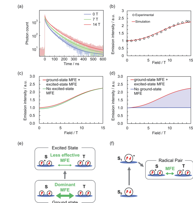
Fig. 4 (a) Simulated and experimental monomer emission decays at 0, 7, and 14 T. ^{31} (b) Simulated and experimental magnetic field dependences of monomer emission intensities. (c) and (d) Simulated monomer emission intensities without considering the MFE on (c) the ground states and (d) the excited states (for details of the simulations, see the ESI ^\dagger ). (e) and (f) Scheme of MFEs on (e) radicals (this system) and (f) conventional ground-state closed-shell molecules.
