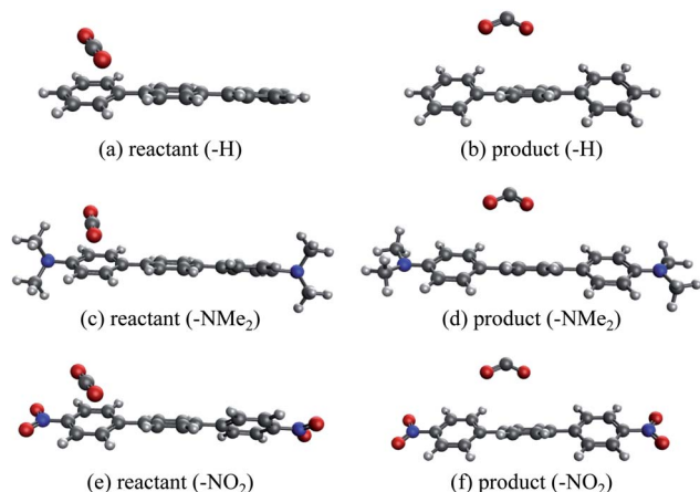
Fig. 13 Optimized structures of unsubstituted and substituted p -terphenyl... \text{CO}_2 radical anion complexes: (a and b) unsubstituted reactant and product complexes; (c and d) \text{NMe}_2 -substituted; (e and f) \text{NO}_2 -substituted.
