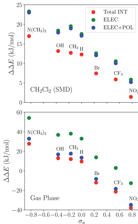
Fig. 14 Substituent effects on the differences in total interaction energies as well as the ELEC and POL components (in \text{kJ mol}^{-1} ) between the reactant and product states. The calculations are performed at the \omega\text{B97X-V}/\text{def2-TZVPD} level of theory. The upper panel shows results in dichloromethane ( \text{CH}_2\text{Cl}_2 ) solvent described by SMD and the lower panel shows gas-phase results. The x-axis shows the Hammett parameter of each substituent group.
