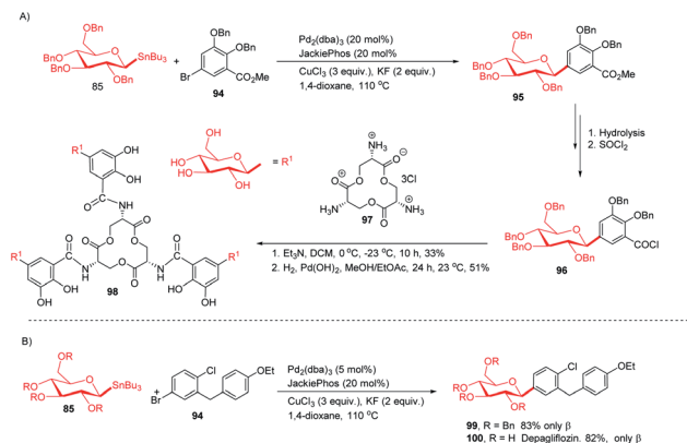
Scheme 28 (A) C-Glycosides via intermolecular Stille-coupling using aryl halides (B) applications of C-glycosides.
