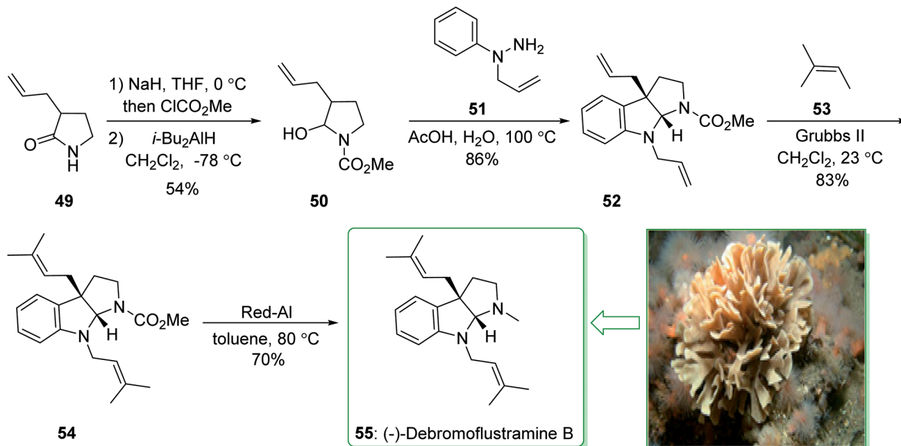
Scheme 7 Formal synthesis of (-)-debromoflustramine B (55).
