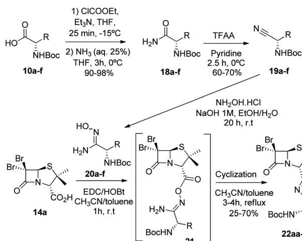
Scheme 4 Synthesis of 1,2,4-oxadiazoles from 6,6-dibromopenicillanic 14a and amidoximes 20a–f .
