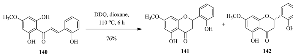
Scheme 50 Synthesis of 5,2'-dihydroxy-7-methoxyflavone and flavanone.
