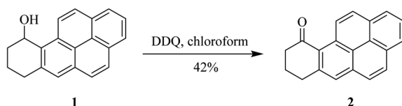
Scheme 3 Benzylic alcohol oxidation by DDQ.
