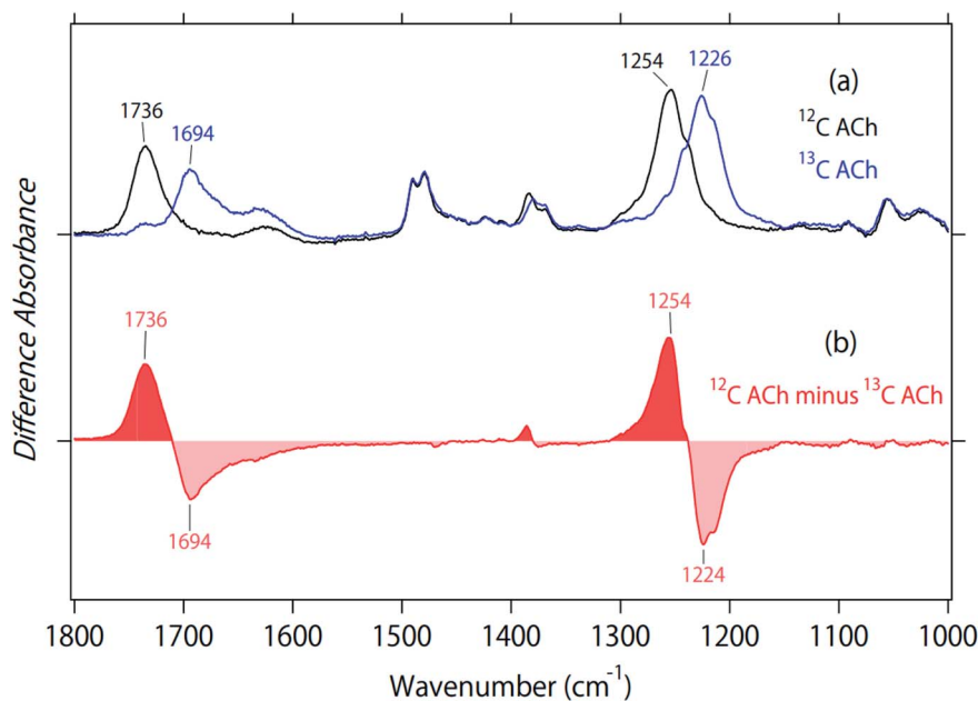
Fig. 4 (a) Absorption spectra of unlabeled (black line) and ^{13}\text{C} -labeled (blue line) acetylcholine in aqueous solution. (b) Difference spectrum of (a), in which the blue spectrum is subtracted from the black spectrum.
