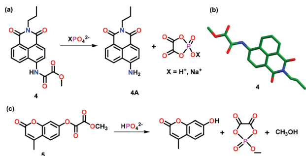
Fig. 3 (a) Chemical drawing of chemosensor 4 and its proposed 'Turn-On' emission mechanism with XPO_4^{2-} ion ( X = H^+ or Na^+ ). (b) Crystal structure of the chemosensor 4. (c) Chemical drawing of chemosensor 5 and its 'Turn-On' emission mechanism with HPO_4^{2-} ions. Adapted from ref. 43 and 44.
