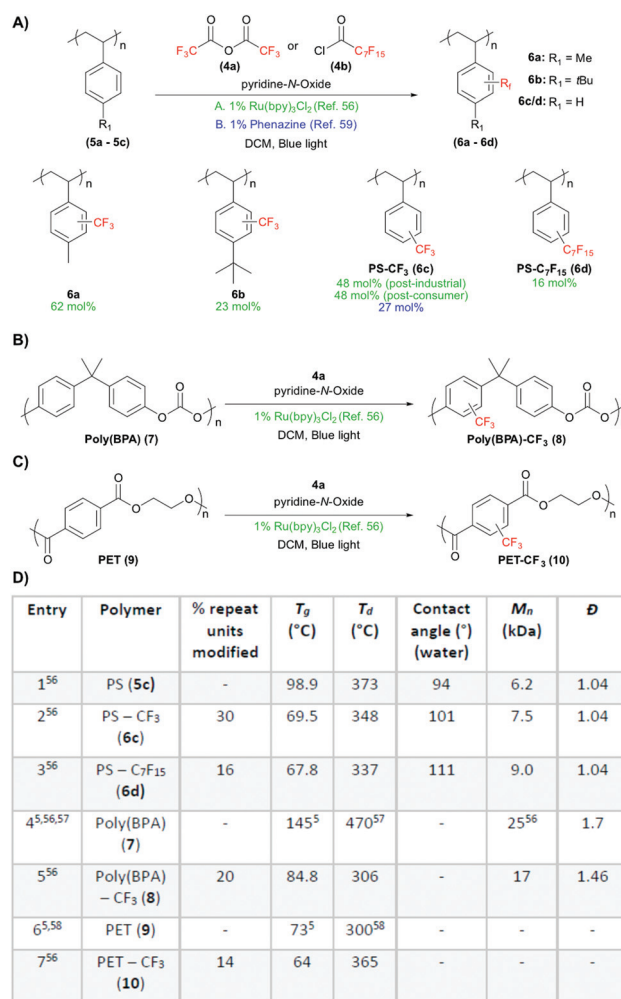
Fig. 2 Trifluoromethylation of various aromatic containing commercial polymers and the resulting polymer properties. (A) Fluorination of polystyrene and polystyrene derivatives (5a–5c) to give fluorinated styrenes (6a–6d). Trifluoromethylation via ruthenium catalyst (green text) was slightly more efficient than via phenazine organic photocatalyst (blue text). Reproduced from ref. 56 with permission from the Royal Society of Chemistry, Copyright 2019. (B) Fluorination of poly(BPA) (7) to give fluorinated poly(BPA) (8). (C) Fluorination of poly(ethylene terephthalate) (9) to give fluorinated PET (10). (D) A table summarizing thermal properties of polymers as well as surface energy through contact angle measurement against water.
