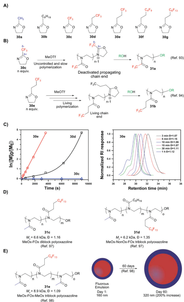
Fig. 6 Oxazoline monomers, polymers, and materials. (A) Select hydrophilic, hydrophobic, and fluorophilic oxazoline monomers 30a–g . (B) Comparison of the polymerization of oxazolines with fluorous groups directly attached to the oxazoline scaffold ( 30c ) vs. those with an ethyl spacer ( 30e ). (C) Left: Comparison of polymerization kinetics between fluorous group and oxazoline heterocycle ( 30c–e ). Right: Size exclusion chromatography (SEC) traces of the 30e homopolymer demonstrating low dispersity. Reproduced from ref. 96 with permission from the American Chemical Society, Copyright 2018. (D) Di and triblock copolymers ( 31c and 31d ) synthesized from methyl, alkyl, or fluorinated oxazoline monomers. (E) Triblock polyoxazoline 31e and the stability of the fluorous emulsions generated from it.
