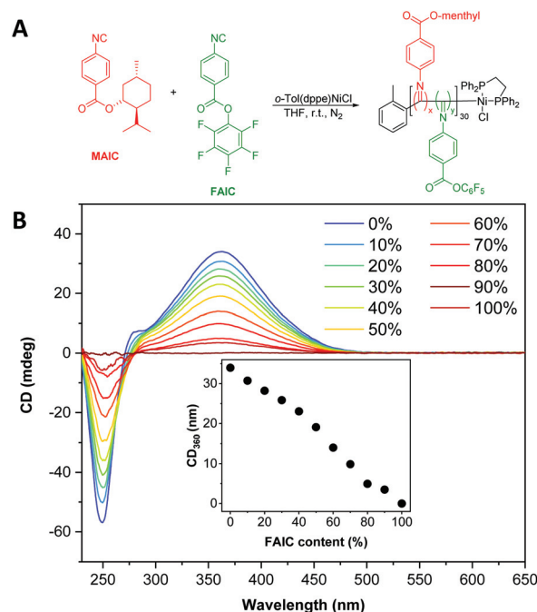
Fig. 1 (A) Synthesis scheme of P( MAIC ) x -co-P( FAIC ) y , where x + y = 30 . (B) CD spectra (THF, 0.5 mg mL -1 ) of P( MAIC ) x -co-P( FAIC ) y copolymers with FAIC content ranging from 0 to 100 mol%.
