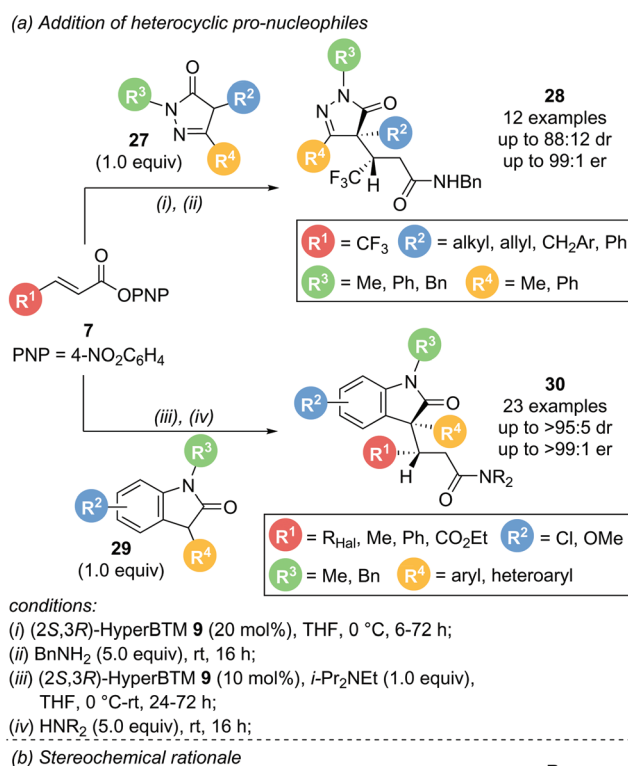
Scheme 7 (a) Conjugate addition of heterocyclic pro-nucleophiles; (b) pre-transition state assembly as stereochemical rational. The scheme illustrates the conjugate addition of heterocyclic pro-nucleophiles to a substituted enone, showing the pre-transition state assembly and the resulting product. (a) Conjugate addition of heterocyclic pro-nucleophiles: The reaction involves a substituted enone (with an \text{Ar} group and a \text{CF}_3 group) reacting with a heterocyclic pro-nucleophile (containing a sulfur atom and a nitrogen atom). The nucleophile attacks the \beta -carbon of the enone, forming a new \text{C-S} bond. The transition state is shown with dashed lines indicating the forming and breaking bonds. The product is a substituted enone with a new heterocyclic ring fused to the original enone system. (b) Pre-transition state assembly as stereochemical rational: This part shows the assembly of the transition state, highlighting the stereochemical control. The transition state is depicted with dashed lines indicating the forming and breaking bonds. The product is a substituted enone with a new heterocyclic ring fused to the original enone system.
