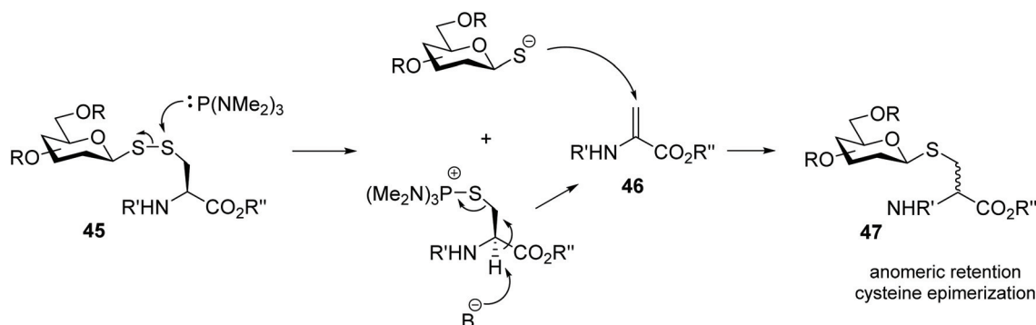
Scheme 15 Proposed \text{S}_\gamma -attack followed by elimination-conjugate addition mechanism of desulfurisation of a disulfide-linked glycosyl cysteine.
