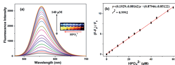
Fig. 4 (a) Fluorescence emission spectra of the N-CDs- \text{Fe}^{3+} complex in the presence of different concentrations of \text{HPO}_4^{2-} from 0 to 140 \mu\text{M} at an excitation wavelength of 450 nm. The inset is the image of the N-CDs- \text{Fe}^{3+} complex in pure water with the increased \text{HPO}_4^{2-} from right to left under UV lamp irradiation at 365 nm. (b) Linear relationship between [(F - F_0)/F_0] and the concentration of \text{HPO}_4^{2-} , where F_0 and F are the fluorescence intensities of the N-CDs- \text{Fe}^{3+} complex at 556 nm in the absence and presence of \text{HPO}_4^{2-} , respectively.
