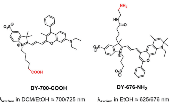
Fig. 2 Benzopyrylium DY-700 and DY-676 used to label BCPs.
