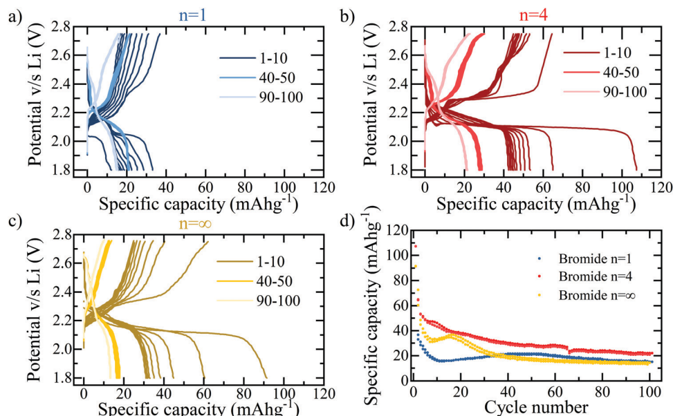
Fig. 4 Galvanostatic cycling of the first insertion mechanism in the reduced potential window of 2.8–1.8 V at a current density of 30 mA g -1 for the layered perovskites (BA) 2 (MA) n-1 Pb n Br 3n+1 probing the lithium insertion process stability in (a) n = 1 (b) n = 4 and (c) the bulk equivalent MAPbBr 3 perovskite structures. (d) Specific capacity of the layered bromide series for the first 100 galvanostatic charge–discharge cycles.
