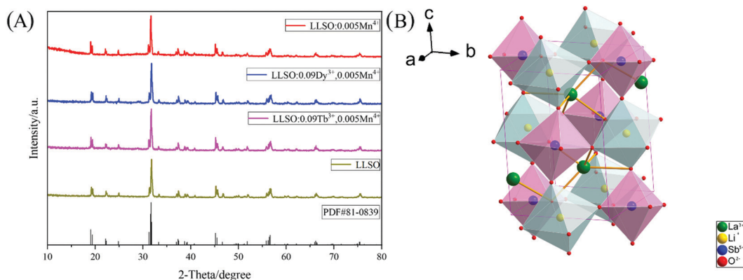
Fig. 1 (A) XRD patterns of \text{LLSO}:0.005\text{Mn}^{4+} , \text{LLSO}:0.09\text{Tb}^{3+}, 0.005\text{Mn}^{4+} , \text{LLSO}:0.09\text{Dy}^{3+}, 0.005\text{Mn}^{4+} and LLSO host. (B) Crystal structure schematic diagram of \text{La}_2\text{LiSbO}_6 .
