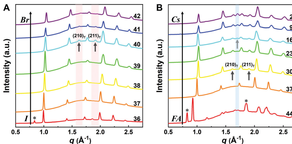
Fig. 5 Integrated circular average of 2D GIWAXS patterns for \text{Cs}_{1/6}\text{FA}_{5/6}\text{Pb}(\text{Br}_x\text{I}_{1-x})_3 films as a function of the Br content (A) and \text{Cs}_\gamma\text{FA}_{1-y}\text{PbBr}_{1/2}\text{I}_{5/2} as a function of the Cs content (B). \delta -FAPbI 3 is marked by *. The black arrows point to the characteristic peaks of the tetragonal phase and the grey arrow refers to the characteristic peaks of orthorhombic phase, i.e., (211) O , (121) O , (103) O .
