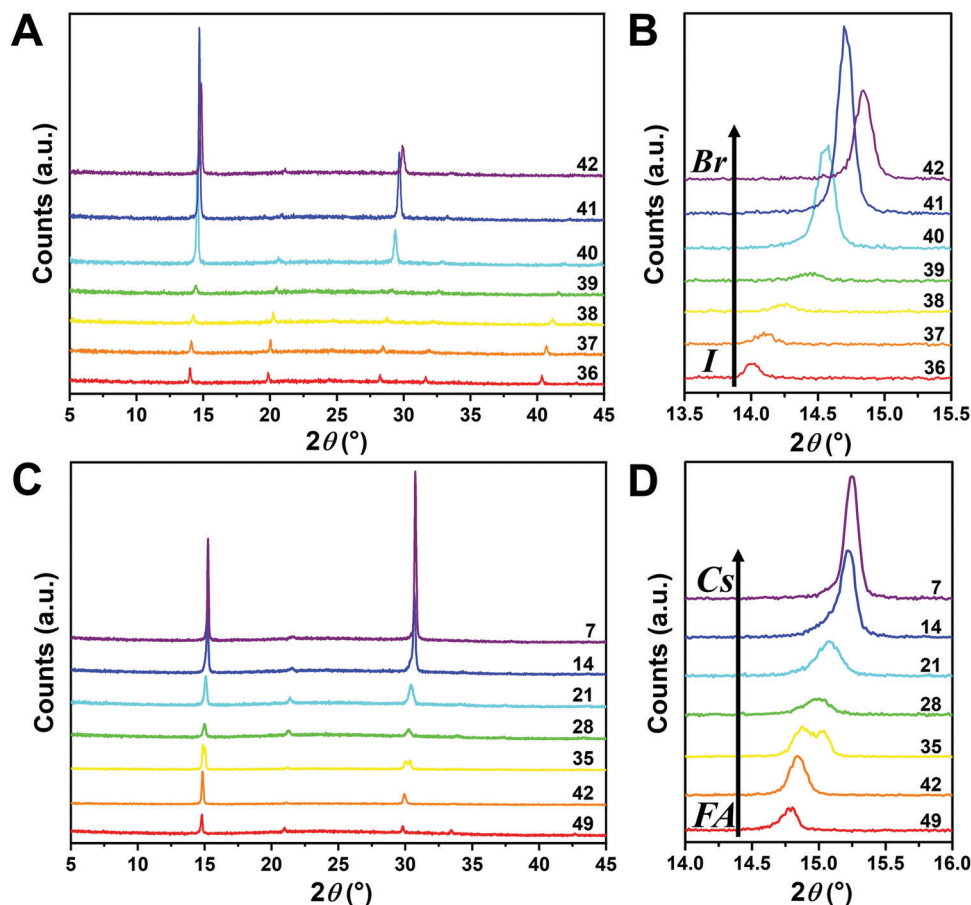
Fig. 4 XRD patterns of \text{Cs}_{1/6}\text{FA}_{5/6}\text{Pb}(\text{Br}_x\text{I}_{1-x})_3 films as a function of the Br content (A and B) and \text{Cs}_\gamma\text{FA}_{1-y}\text{PbBr}_3 as a function of the Cs content (C and D). (B) and (D) are expanded views of the peaks at \sim 14-15^{\circ} in (A) and (C).
