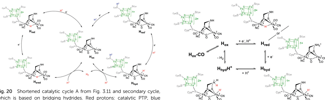
Fig. 21 Schematic representation of the catalytic cycle of [FeFe]-hydrogenase, based on the states observed under whole-cell conditions including the protonated hydride species ( \text{H}_{\text{hyd}}\text{H}^+ ). Figure and caption from ref. 35.
