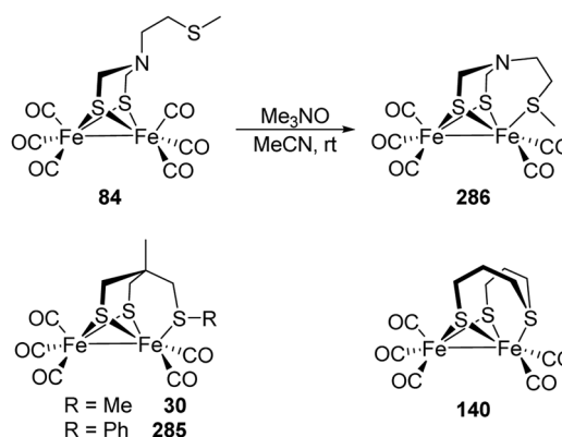
Fig. 86 [2\text{Fe-}3\text{S}] -assemblies carrying a thioether on the dithiolate bridge.
