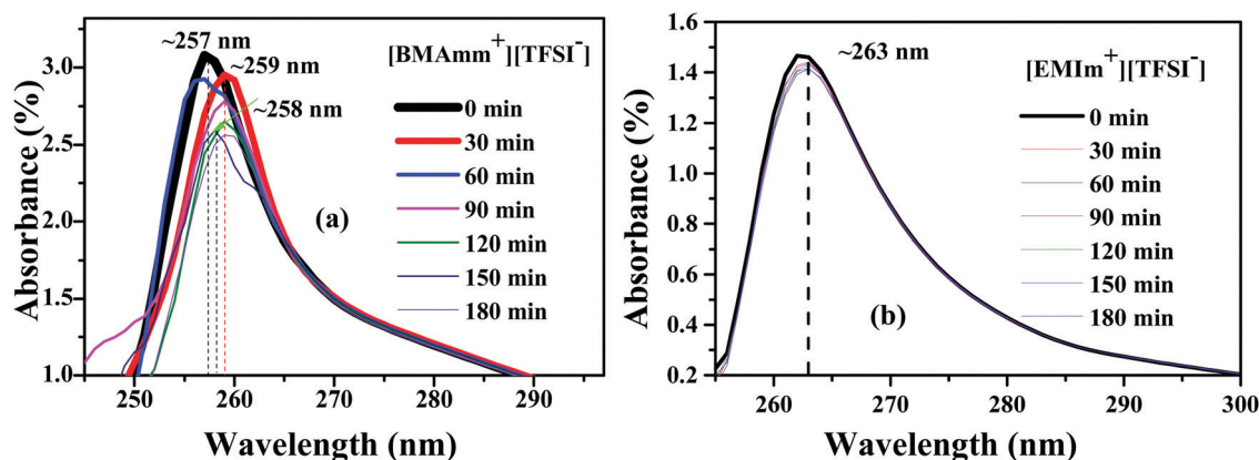
Fig. 4 Absorbance spectra of \text{O}_2^{\bullet-} generation in DMSO in the presence of (a) [BMAm + ][TFSI - ] and (b) [EMIm + ][TFSI - ].
