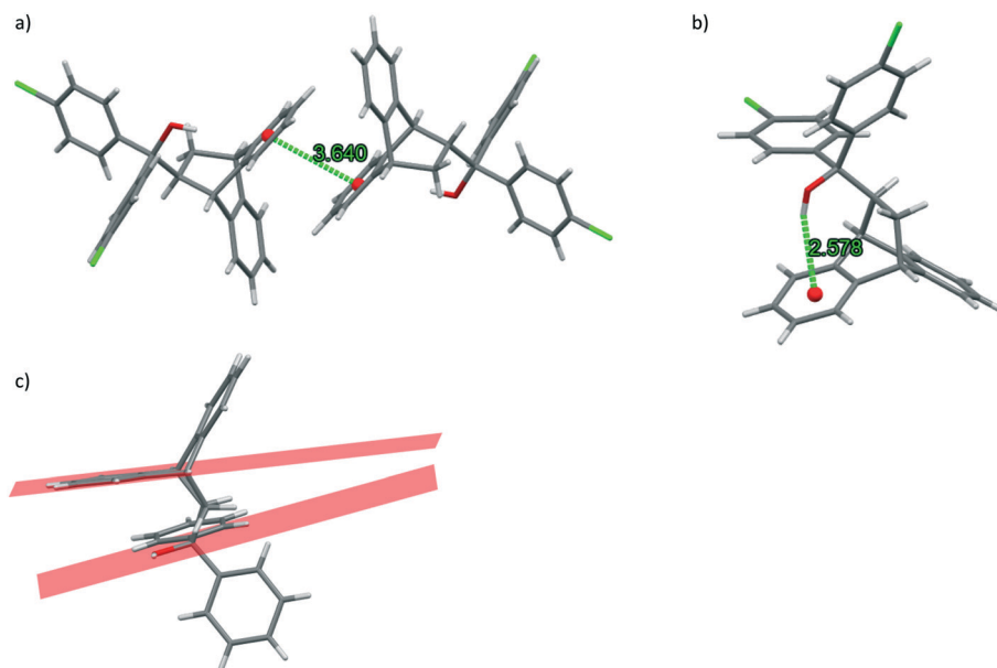
Fig. 3 Host...host a) intermolecular \pi\cdots\pi (in H2-p-Xy ) and b) intramolecular OH \cdots\pi (in H2-EB ) interactions; c) the calculated planes (red) of the adjacent fused aromatic ring system and the C-O-H group of H1 in H1-o-Xy ; guest molecules are not shown here.
