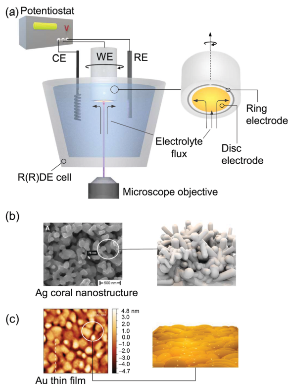
Fig. 2 (a) EC-Raman/SER spectroscopy coupled to a rotating (Ring) disc electrode (R(R)DE) electrochemical setup. A microscope objective focusses the exciting laser onto the disc working electrode (WE). Rotation imposes a defined electrolyte flux. Potentials at the ring electrode can be separately adjusted. CE and RE denote counter and reference electrodes, respectively. (b) SEM image of a plasmonic Ag electrode obtained via electrochemical roughening. Reprinted from ref. 88. (c) AFM image of a nanoscopically rough Au electrode for EC-SEIRA spectroscopy obtained via electroless deposition on a Si prism. Reprinted from ref. 104.
