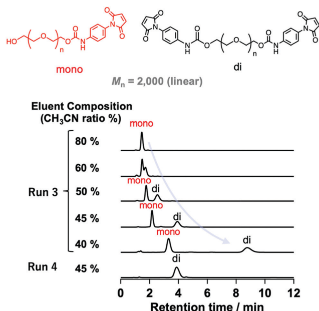
Fig. 2 HPLC profiles of modified PEGs ( M_n = 2000 ) with different numbers of N -aryl MA groups (Runs 3 and 4 in Table 1) using different eluent compositions (values shown are the vol% of acetonitrile in water) at a flow rate of 1.0 mL min ^{-1} on a C18 column at 30 °C using a UV detector.
